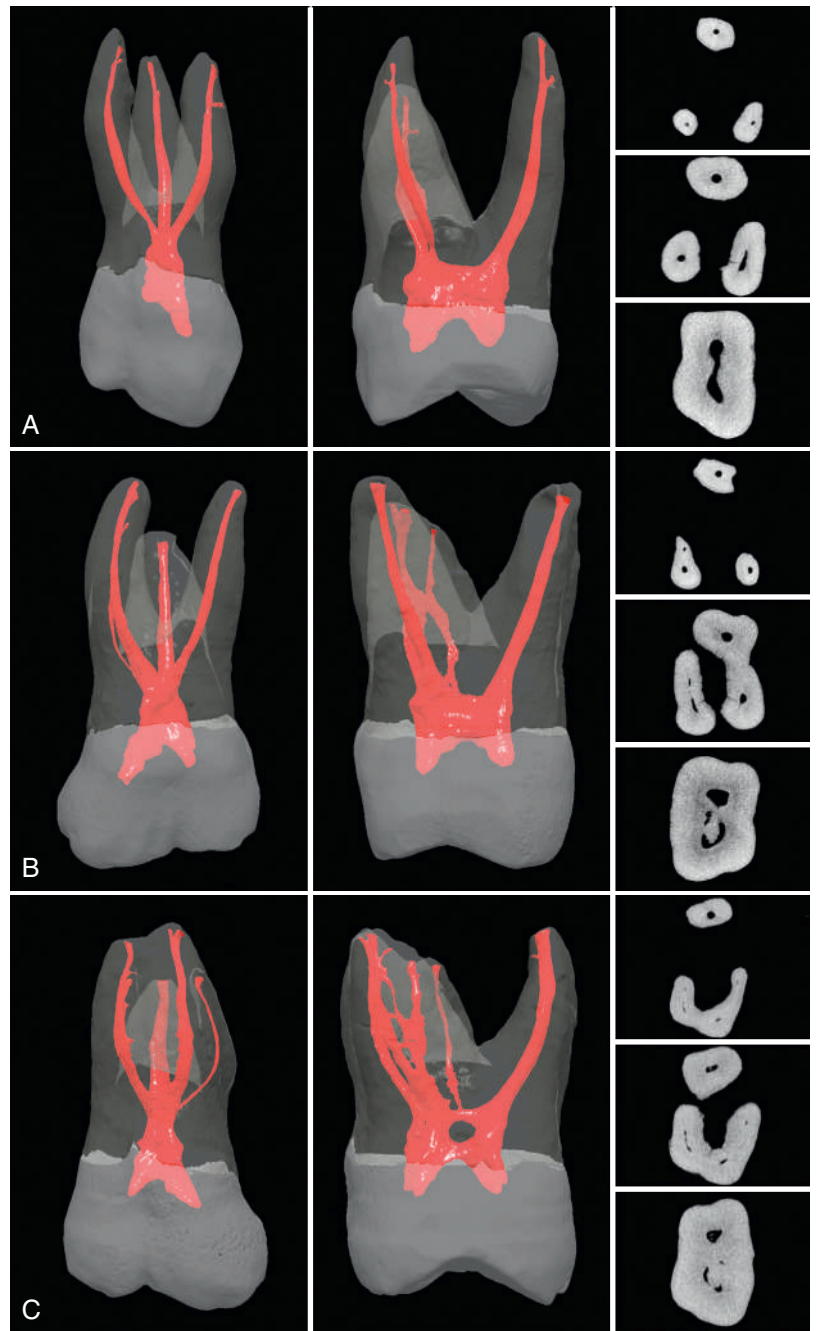
Fig. 7.59 \mu CT scans of maxillary first molars. A , Common anatomic presentation showing accessory/lateral canals. B , First molar with four canals, with mesiobuccal and mesiopalatal sharing an anastomosis in the mid-root. C , Maxillary molar with four pulp horns, five canals, and significant anastomoses between the canals. All teeth are shown from both a buccal (vestibular) and a proximal perspective, along with the cross-sectional anatomy at the coronal, middle, and apical levels.
